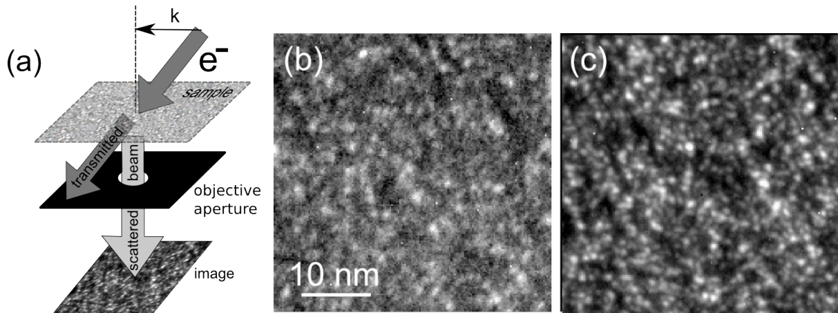
Figure 1. (a) Schematic drawing of the FEM technique using tilted illumination. Examples of tilted dark-field images showing low (b) and high values (c) of the normalized variance.
