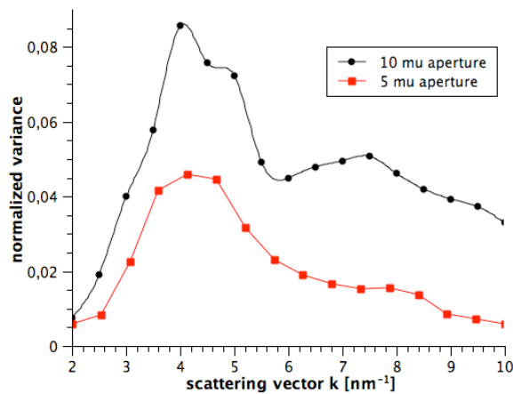
Figure 4. Plot of V(k) calculated from sets of dark-field images taken with different objective apertures (5 and 10 \mu\text{m} in diameter).
