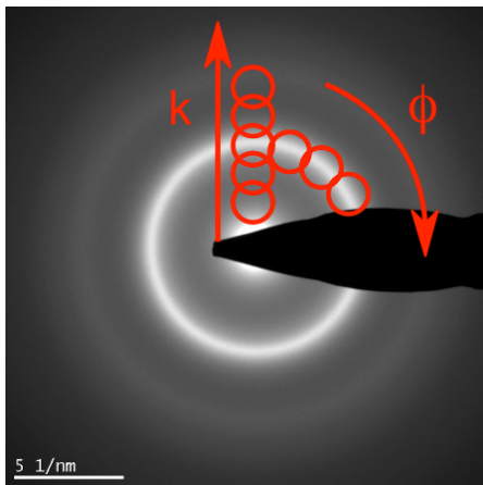
Figure 2. Diffraction pattern of CuZrAlAg bulk metallic glass is characterized by diffuse rings. For the FEM analysis a set of dark-field images is taken by varying the scattering vector k and the angle \phi . The rings illustrate the different positions of the objective apertures used to form the dark-field images.
