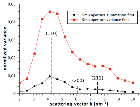
Figure 3. Plot of the normalized variance V(k) of the intensity of images taken with a 5 \mu\text{m} objective aperture. The two curves differ by the method of averaging over the angle \phi . Lower values of V(k) are obtained by calculating V of images summed first over \phi . The position of structure factors (hkl) of B2 ordered CuZr is indicated.
