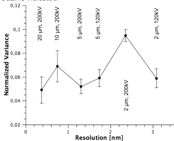
Figure 5. Plot of the normalized variance as a function of the resolution determined by the size of the objective aperture and the acceleration voltage.
