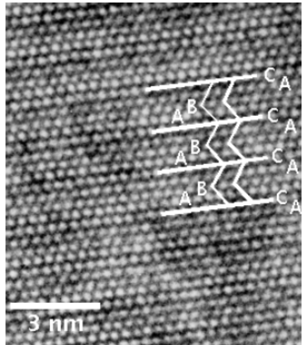
Fig. 3: HRTEM image of the Laves phase in the as-cast alloy showing the unfaulted ABAC stacking sequence of Co 2.1 Ti 0.9 .
