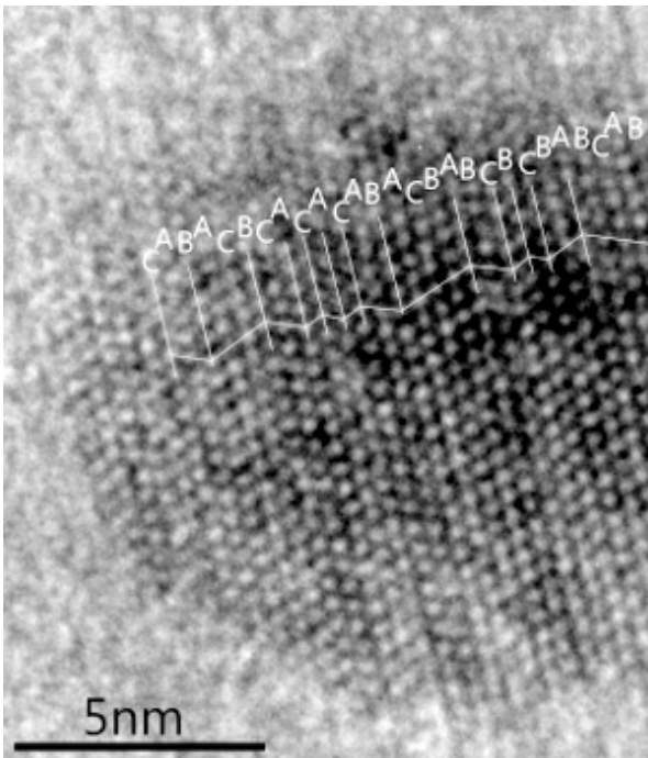
Fig. 2: HRTEM image of a nanocrystal showing Kagome layers with frequently occurring stacking faults.
