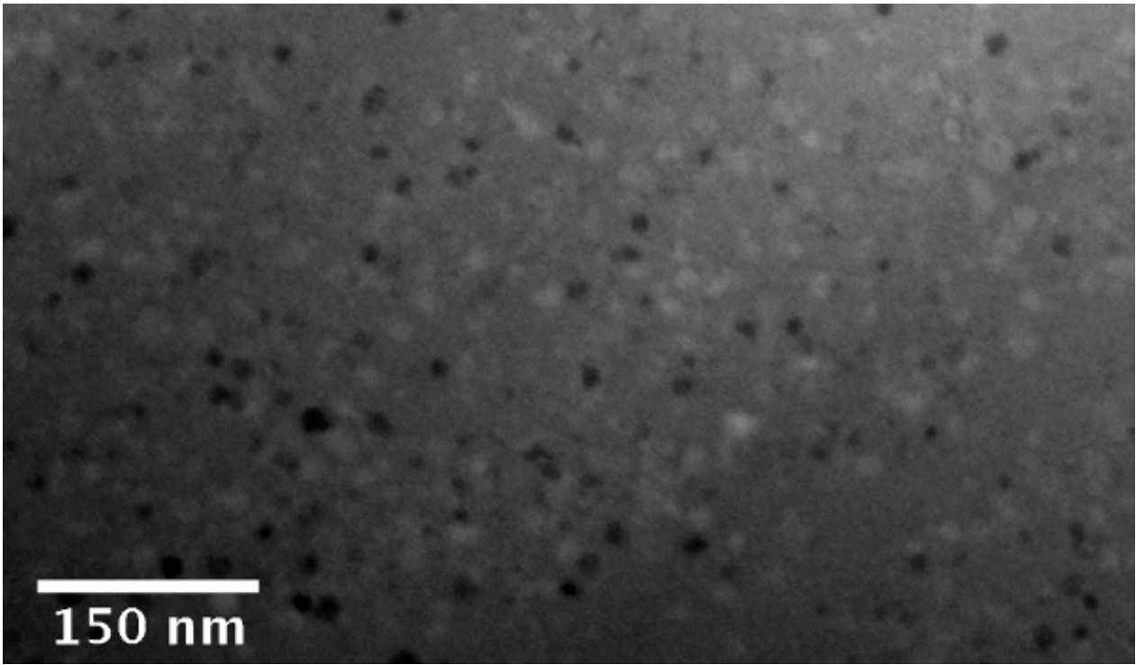
Fig. 1: BF image of the amorphous phase of the Co 3 Ti alloy with embedded nanocrystals formed by dynamic crystallization. The nanocrystals show bright and dark contrast relative to the contrast of the amorphous phase.
